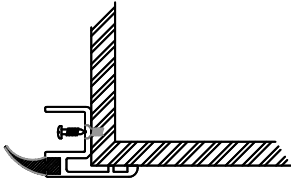
30DRS612-ONE PIECE GUIDE 30DRS316S-SIDE SEAL
