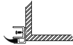
30DRS314-STAINLESS STEEL TRACK 30DRS342-SEAL HOLDER "L" 30DRS316S-SIDE SEAL 30DRS350B-INFILL STRIP
