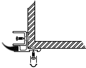
30DRS314-STAINLESS STEEL TRACK 30DRS347-FRAME SURROUND SEAL HOLDER 30DRS316S-SIDE SEAL 30DRS350B-INFILL STRIP
