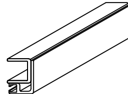
30DRS347B-ONE PIECE GUIDE WITH GROOVE 30DRS350B-INFILL STRIP 30DRS316S-SIDE SEAL
