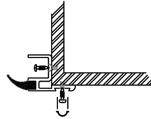
30DRS347B-ONE PIECE GUIDE WITH GROOVE 30DRS350B-INFILL STRIP 30DRS316S-SIDE SEAL
