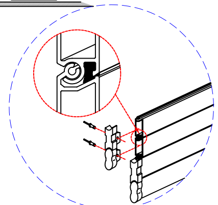
INTERGRATED RUBBER JOINT SEAL INTERLOCKING BALL AND SOCKET SLATS MECHANICALLY FASTENED END LOCKS
