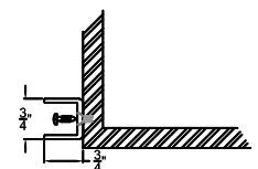
INTERGRATED RUBBER JOINT SEAL INTERLOCKING BALL AND SOCKET SLATS MECHANICALLY FASTENED END LOCKS
