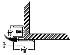
ONE PIECE GUIDE
