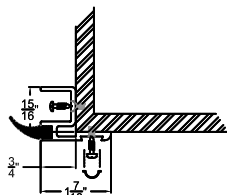
ONE PIECE GUIDE With Groove
