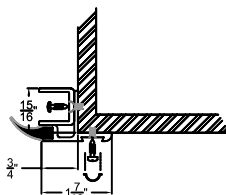
STAINLESS STEEL TRACK WITH T-TRIM
