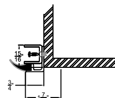
STAINLESS STEEL TRACK WITH L-TRIM
