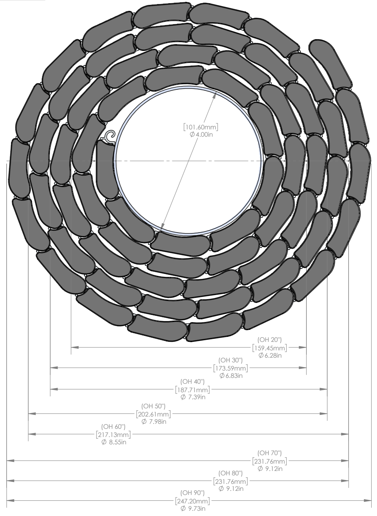
2EB 4" COUNTERBALANCE
