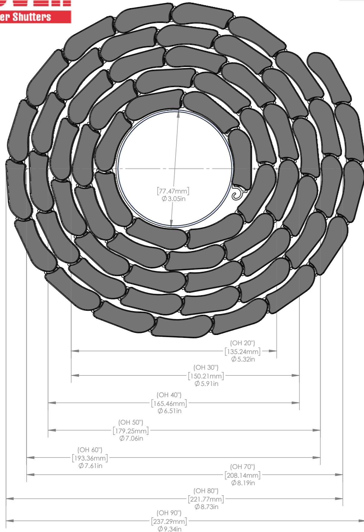
2EB 3" COUNTERBALANCE
